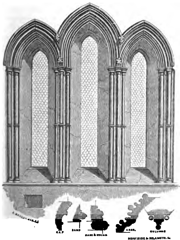
90. Polebrook, Northants, c. 1220.
